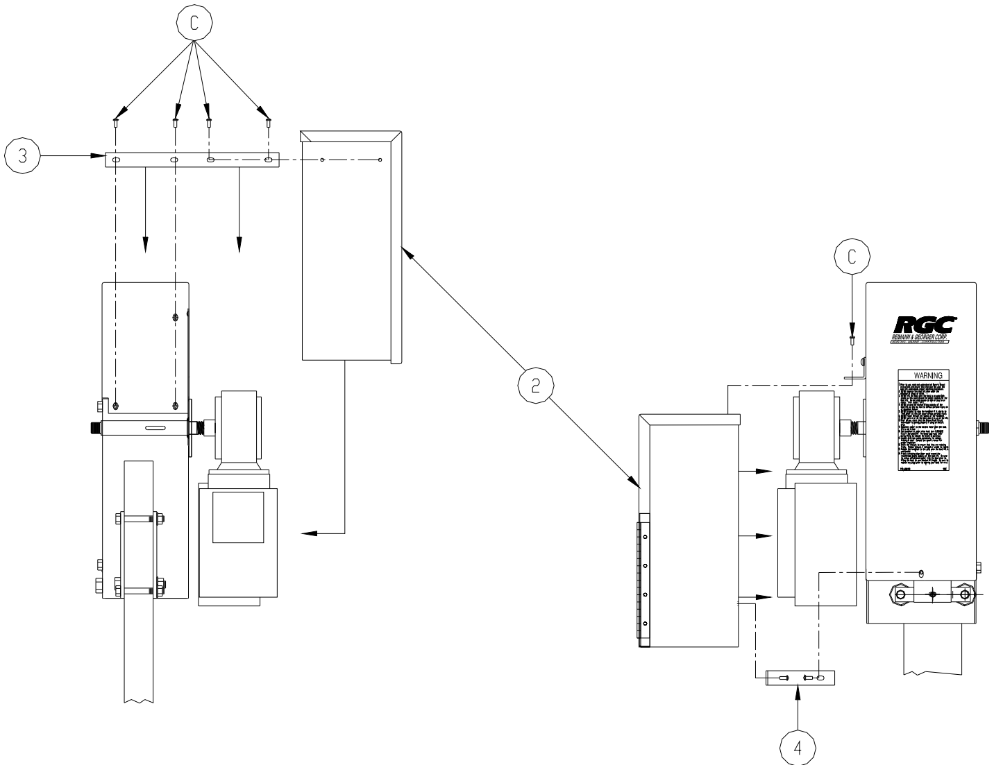
Figure 2-2 VL Direct Drive Guard Installation
